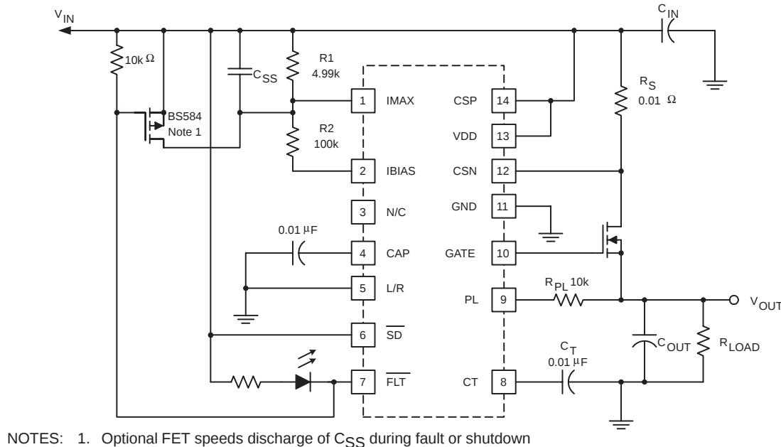
Figure 5. Application Circuit
